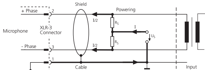
Fig. 1 Input with transformer (or balanced, ungrounded transformerless input)
